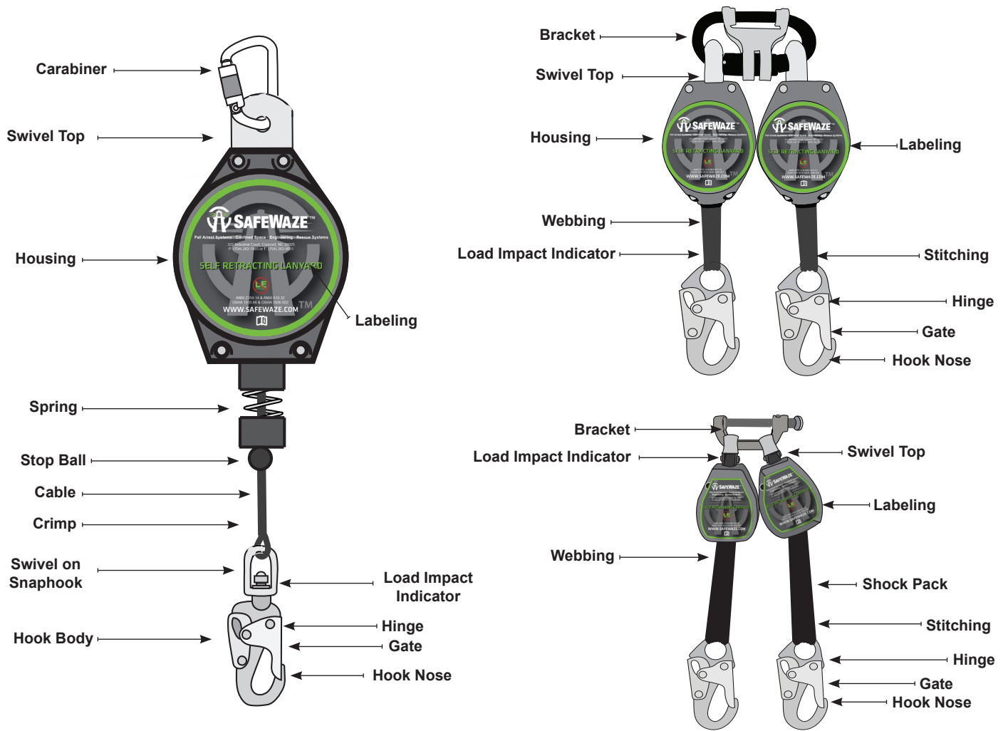
FIGURE 18 - INSPECTION DIAGRAMS
